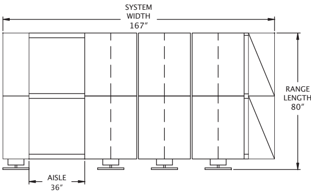
Top View of System Range
