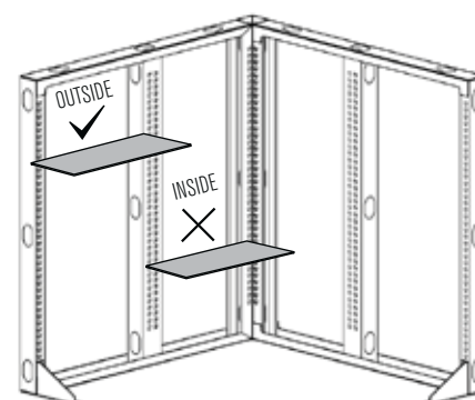
Placement of straight shelves on a corner frame (outsides only)
